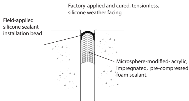
HORIZONTAL-PLANE APPLICATION
