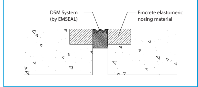
Figure 1: Emcrete Used as Expansion Joint Nosing Material
