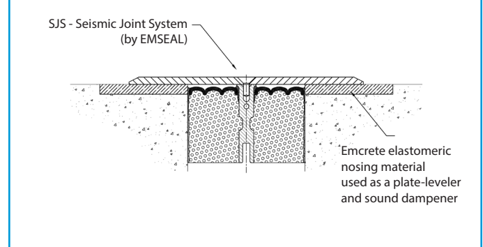
Figure 3: Emcrete Used with SJS System as a Plate-Leveler and Sound Dampener
