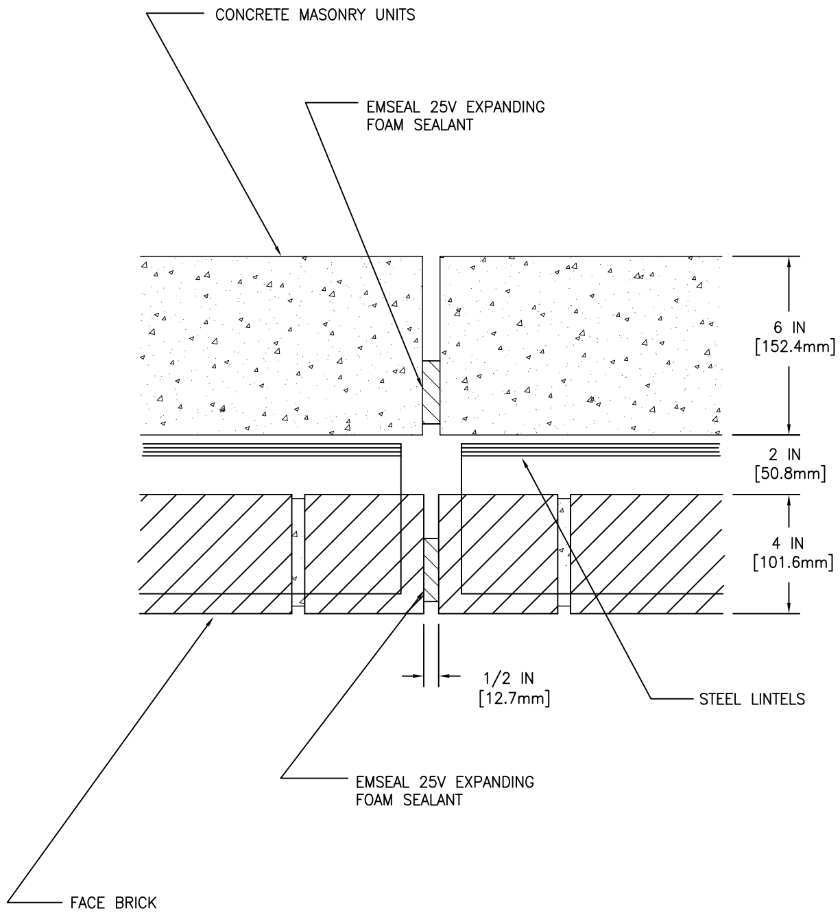
PLAN VIEW
